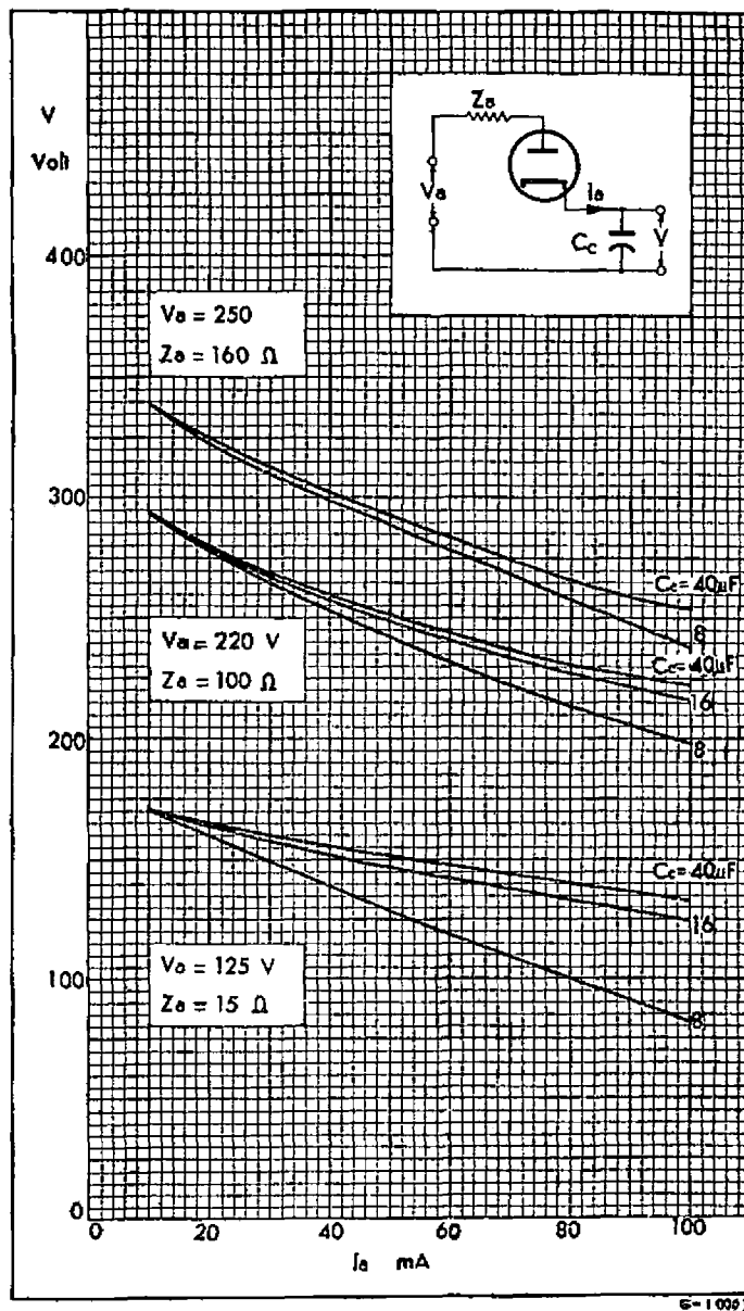
Fig. 1 — Operation Characteristics
