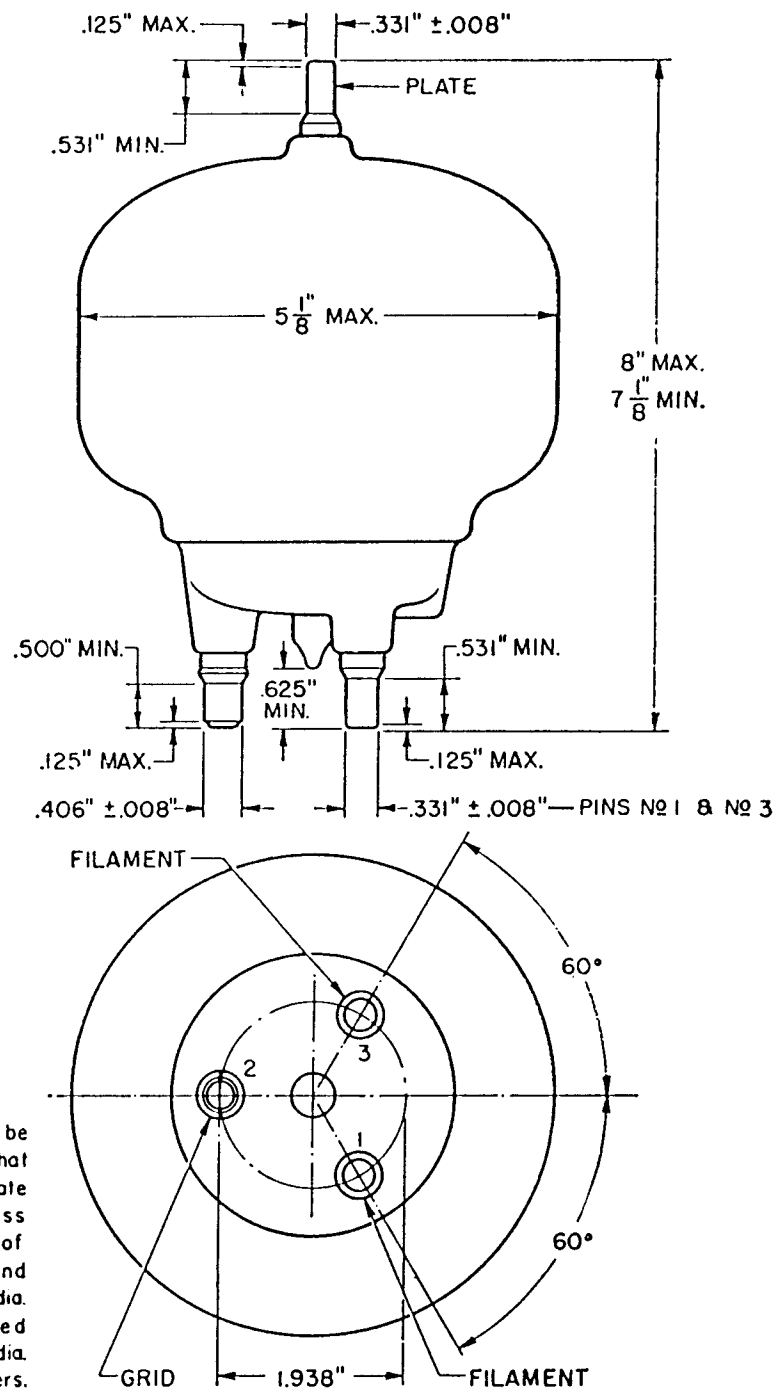
DIMENSIONS—ML-357B
