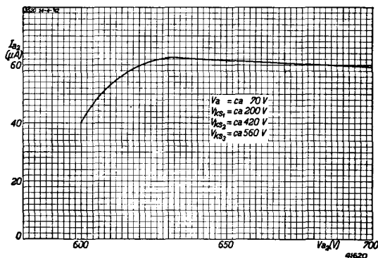
I_a/V_a characteristics of the 3520 secondary-emission cell.
