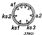
Electrode connections and maximum dimensions in millimetres.
