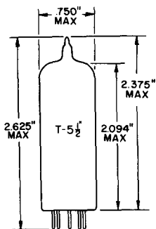
GLASS BULB SMALL BUTTON MINIATURE 7 PIN BASE E7-1 OUTLINE DRAWING JEDEC 5-3
