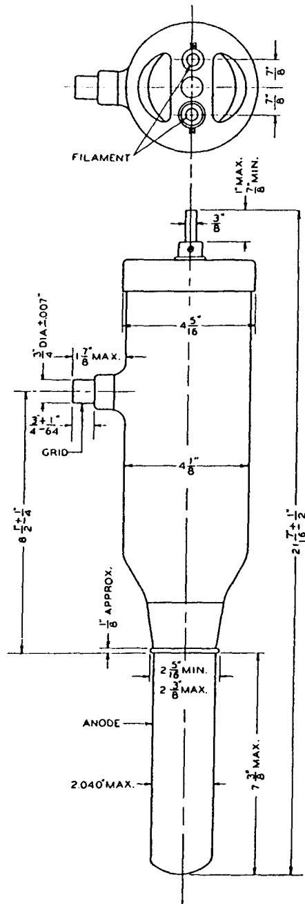
DIMENSIONS—ML-342A
