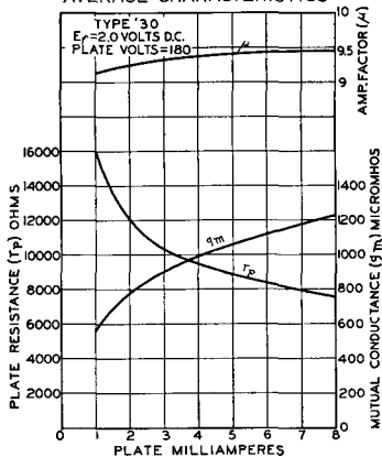
AVERAGE CHARACTERISTICS
