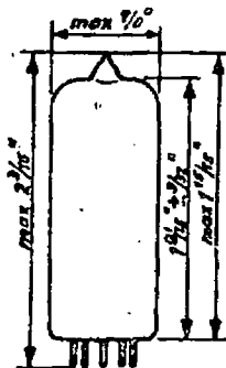
Tube outline
