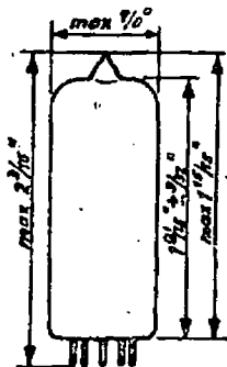
Tube outline
