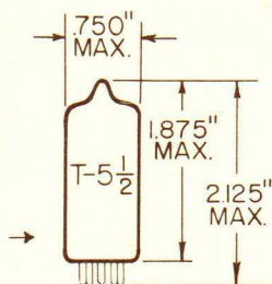
GLASS BULB MINIATURE BUTTON 7 PIN BASE ET-1 OUTLINE DRAWING JEDEC 5-2
