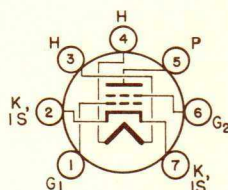
BOTTOM VIEW PINNING DIAGRAM JEDEC 7EW
