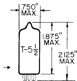
GLASS BULB MINIATURE PUTTON 7 PIN BASE E7-1 OUTLINE DRAWING JEDEC 5-2
