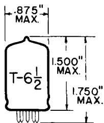
GLASS BULB MINIATURE BUTTON 9 PIN BASE E9-1 OUTLINE DRAWING JEDEC 6-1
