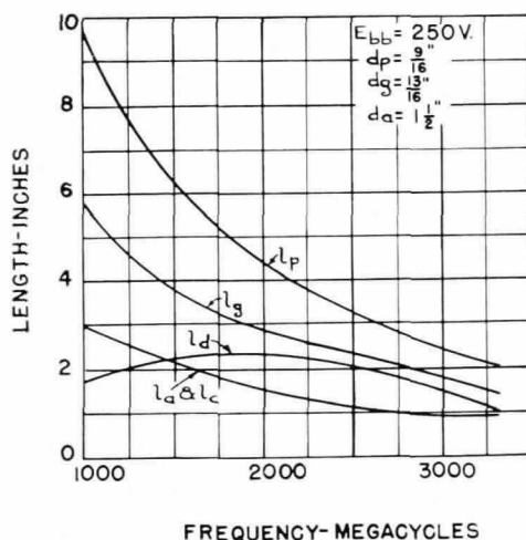
Fig. 5—Curves of Approximate Dimensions for Circuit Shown in Fig. 4
