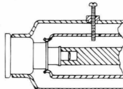
Fig. 3D—Fixed-Probe Feedback, Folded-Back Cavity
