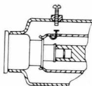
Fig. 3B—Loop-Probe Feedback, Folded-Back Cavity K-5109739
