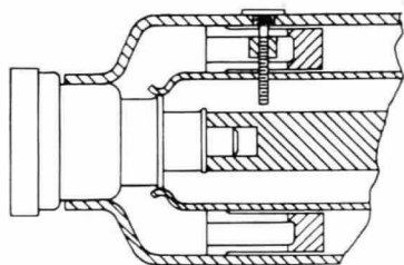
Fig. 3A—Movable Probe Feedback, Folded-Back Cavity
