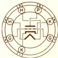
BOTTOM VIEW MINIATURE BUTTON 7 PIN BASE TEG
