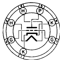
BOTTOM VIEW MINIATURE BUTTON 7 PIN BASE 7EG
