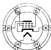
MEDIUM 6 PIN BASE
