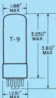
GLASS BULB INTERMEDIATE SHELL B8-6 OR SHORT INTERMEDIATE SHELL B8-58 8 PIN OCTAL OUTLINE DRAWING JEDEC 9-33 OR 9-44
