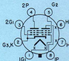
BOTTOM VIEW BASING DIAGRAM JEDEC 8BU
