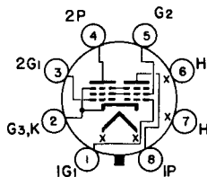
BOTTOM VIEW BASING DIAGRAM JEDEC 8BU
