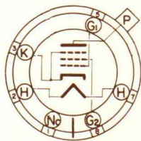
BOTTOM VIEW SHORT MEDIUM-SHELL 8 PIN OCTAL 5BT
