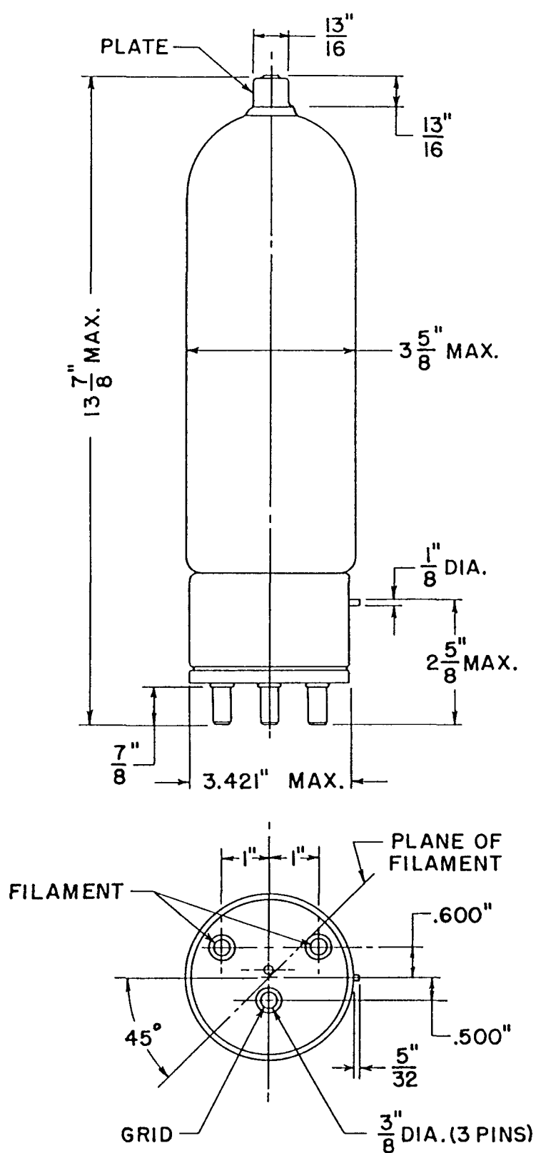
DIMENSIONS—ML-241B
