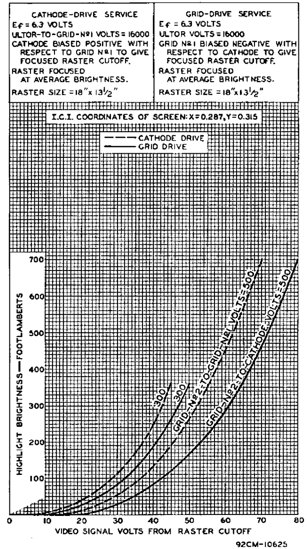
Fig. 5 - Average Drive Characteristics of Type 23MP4.
