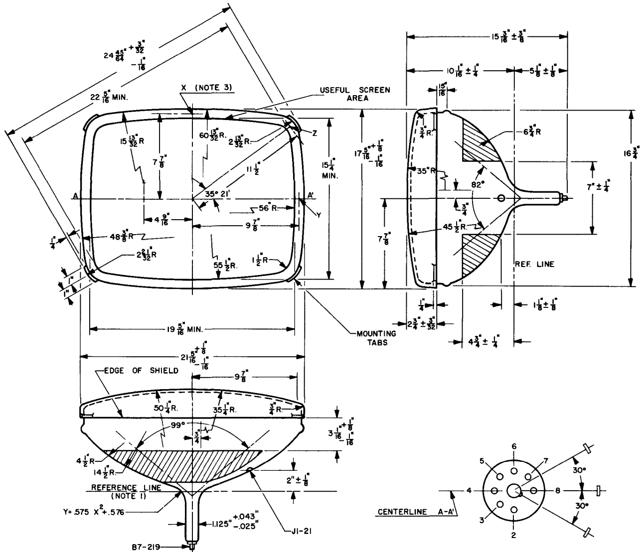
BOTTOM VIEW OF BASE (NOTE 2)
