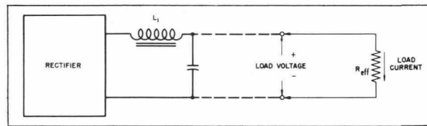
Fig. 1. Rectifier with Choke-Input Filter
