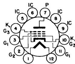
BOTTOM VIEW BASING DIAGRAM JEDEC 12 BJ
