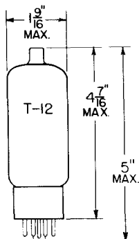
GLASS BULB
