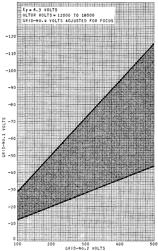
Fig. 1 - Raster Cutoff Range for Type 21CEP4 in Grid-Drive Service.
