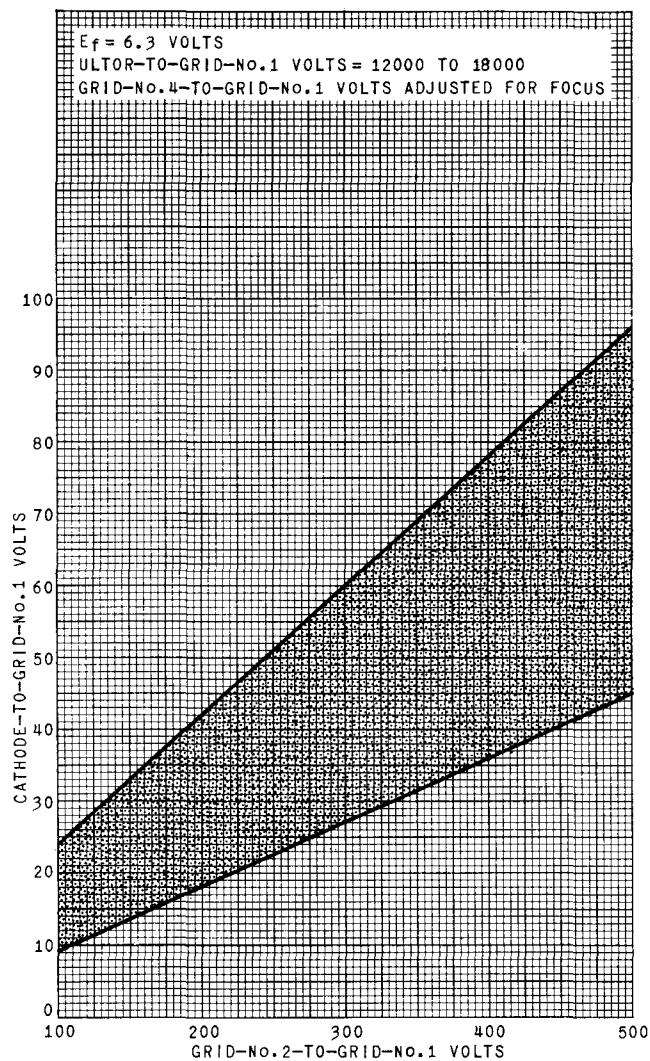
Fig. 2 - Raster Cutoff Range for Type 21CEP4 in Cathode-Drive Service.
