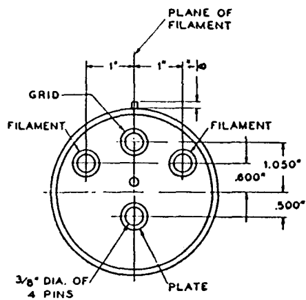
DIMENSIONS—ML-212E
