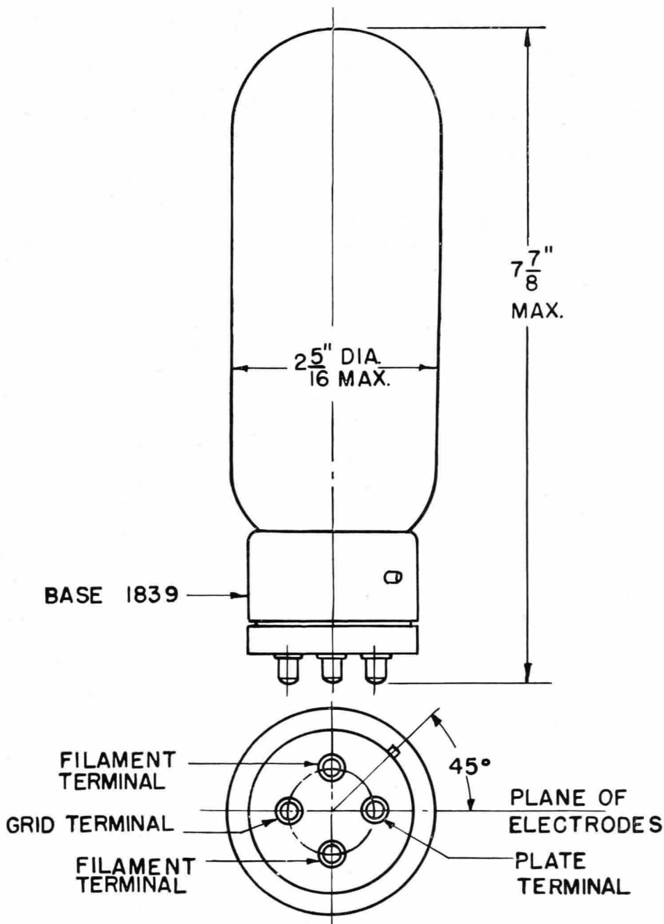
GL-211 OUTLINE
