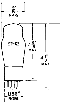
GLASS BULB
