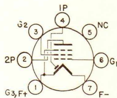
BOTTOM VIEW BASING DIAGRAM JEDEC 6BW
