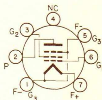
BOTTOM VIEW BASING DIAGRAM JEDEC 6AR
