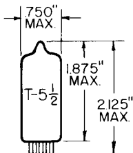
GLASS BULB MINIATURE BUTTON 7 PIN BASE ET-1 OUTLINE DRAWING JEDEC 5-2
