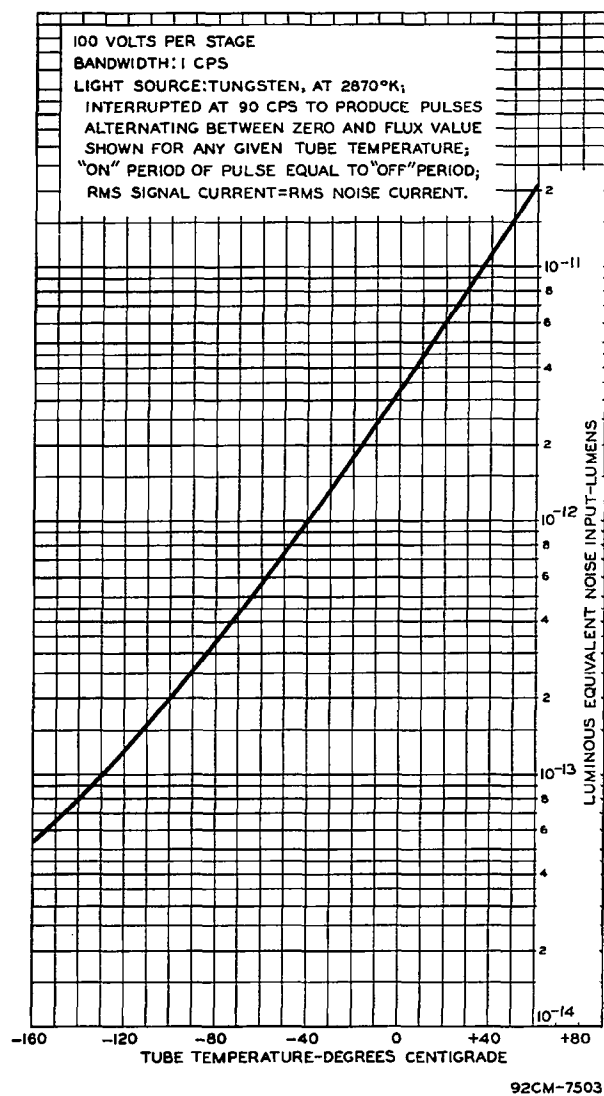
Fig. 7 - Equivalent Noise Input Characteristic of Type 1P28.
