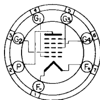
BOTTOM VIEW MINIATURE BUTT 7 PIN BASE 70C
