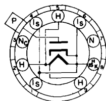
BOTTOM VIEW SMALL BUTTON 9 PIN BASE 9LX
