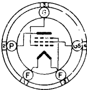
5K BOTTOM VIEW 1F4
