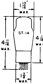
MEDIUM 5 PIN BASE 1F4
