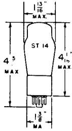
MEDIUM 7 PIN OCTAL BASE 1F5G
