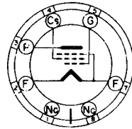
G 6X BOTTOM VIEW 1F5G
