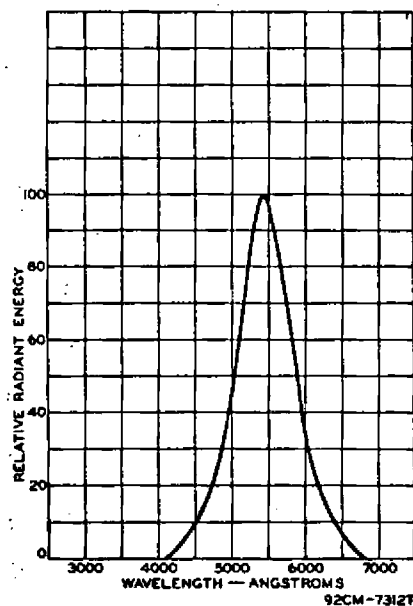
Fig. 4 - Spectral-Energy Emission Characteristic of Phosphor P2.
