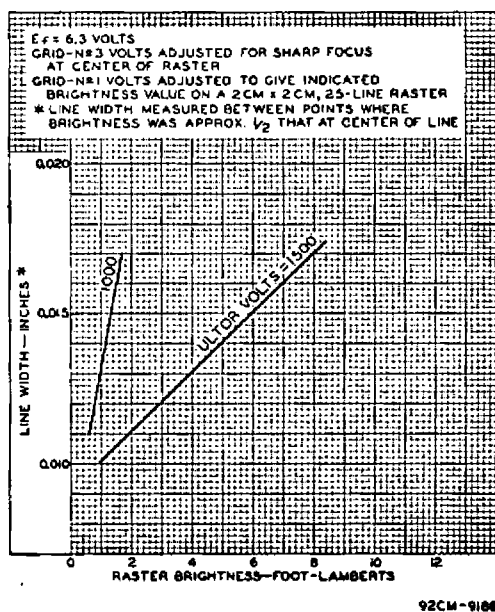
Fig. 9 - Average Characteristics of Type 1EP11.
