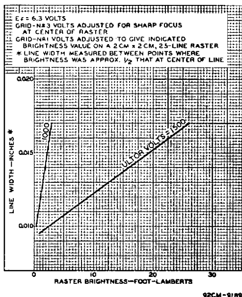
Fig. 6 - Average Characteristics of Type 1EP2.
