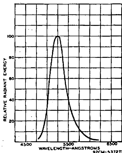
Fig. 1 - Spectral-Energy Emission Characteristic of Phosphor P1.
