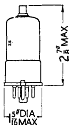
1A7GT
