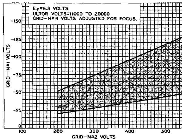
Fig. 2 - Raster-Cutoff-Range Chart for Type 19XP4 in Grid-Drive Service.
