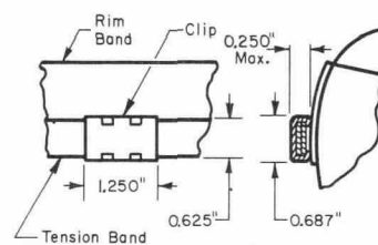
CLIP DETAIL
