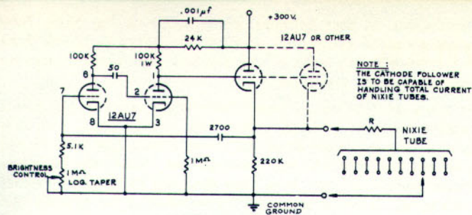
Figure 6—Nixie Tube Dimming Circuit
