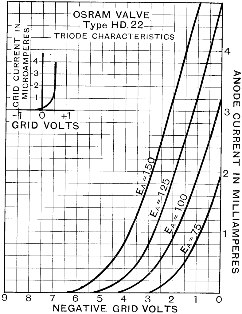
TRIODE CHARACTERISTIC CURVES OF AVERAGE VALVE.
