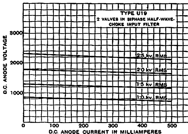
CHARACTERISTIC CURVES OF AVERAGE VALVE.
