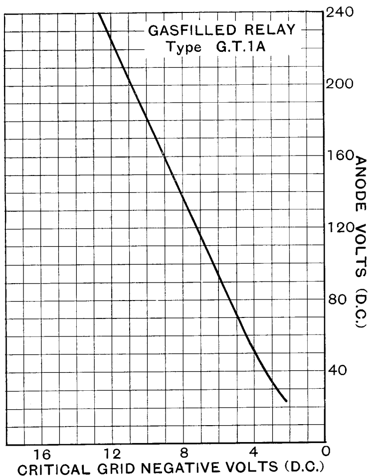
CHARACTERISTIC CURVE OF AVERAGE VALVE.
