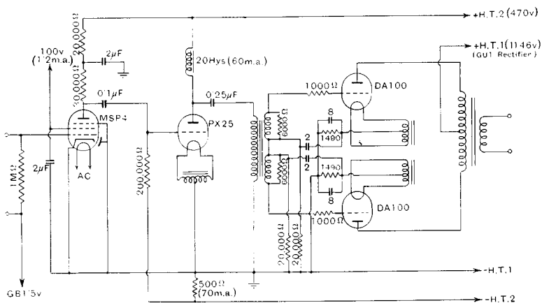
TYPICAL CIRCUIT FOR 90 WATT AMPLIFIER.
