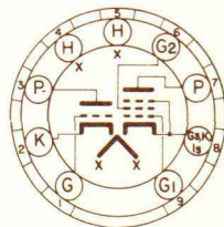
BOTTOM VIEW MINIATURE BUTTON 9 PIN BASE 9 ME
