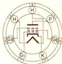
BOTTOM VIEW MINIATURE BUTTON 7 PIN BASE TCC
