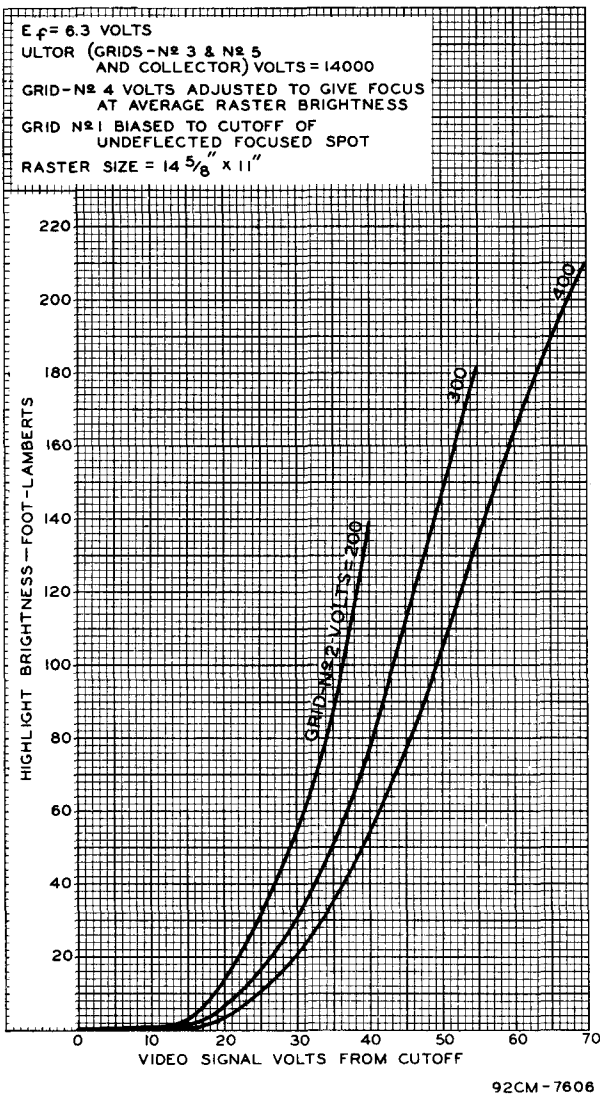
Average Grid-Drive Characteristics of Type 17TP4.
