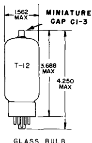
GLASS BULB SHORT MEDIUM SHELL 5 OR 6 PIN OCTAL WITH EXTERNAL BARRIERS 66-122 OR 65-190
