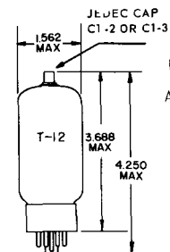
GLASS BULB SKIRTED MINIATURE SHORT MEDIUM-SHELL 6 PIN OCTAL B6-122, B6-148 OR 7 PIN OCTAL B7-111, B7-119 OR B5-190 ← OUTLINE DRAWING JEDEC 12-51
