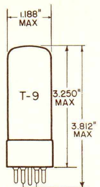
GLASS BULB SHORT INTERMEDIATE SHELL 5 PIN OCTAL WITH EXTERNAL BARRIERS B5 - 85 OUTLINE DRAWING JEDEC 9-44
