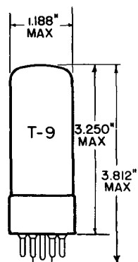
GLASS BULB SHORT INTERMEDIATE SHELL 5 PIN OCTAL WITH EXTERNAL BARRIERS B5-85 OUTLINE DRAWING JEDEC 9-44
