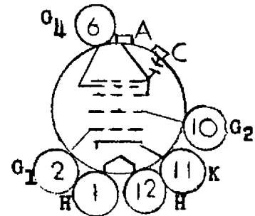
SMALL SHELL DUODECAL 6 PIN BASE B6-63-NOTE-2-
