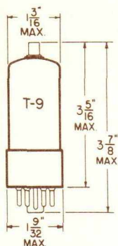
GLASS BULB SKIRTED MINIATURE CAP
